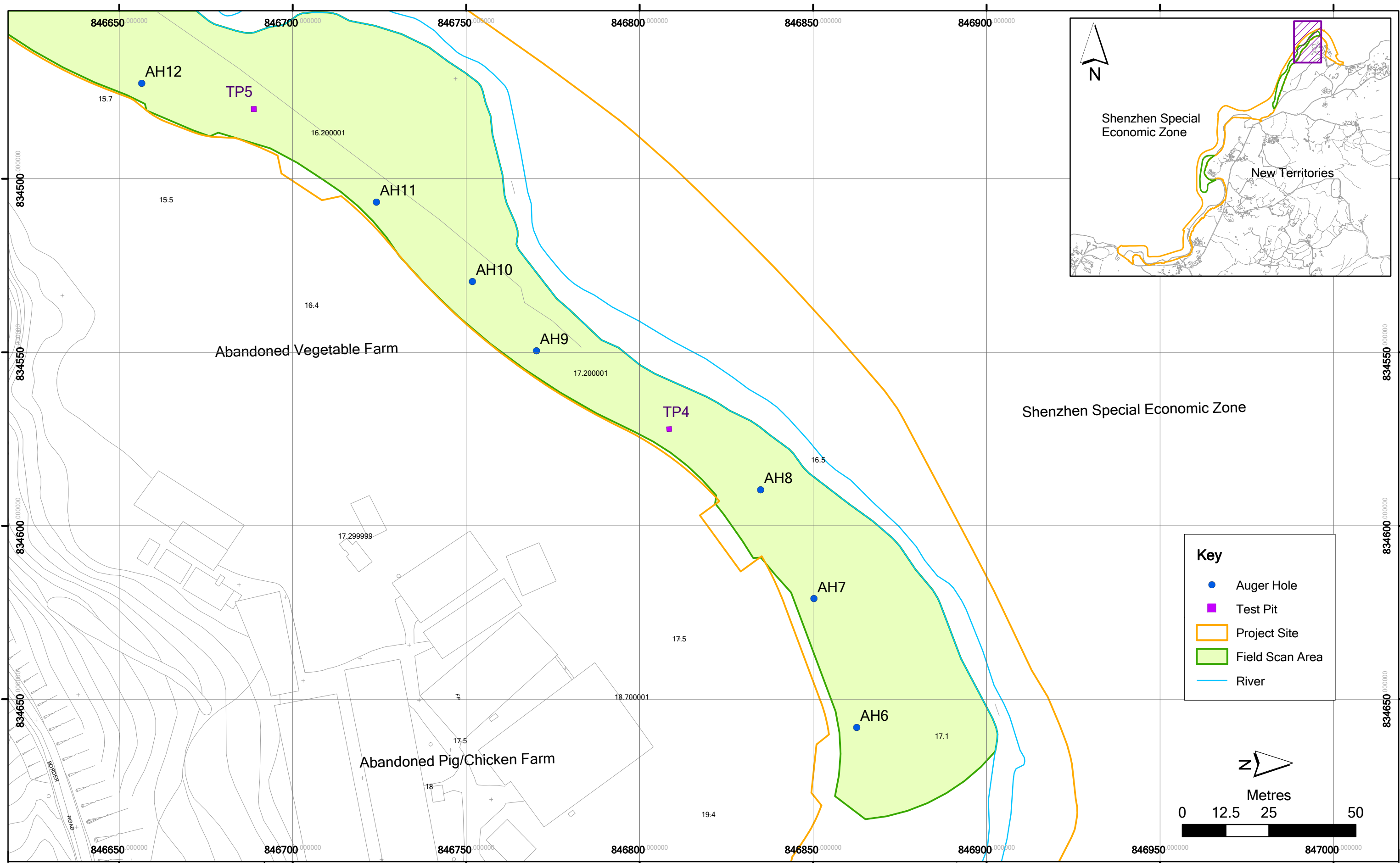
Figure 11.16 Layout Plan for Test Pits and Auger Holes Location and Topography of Pak Fu Shan Section
